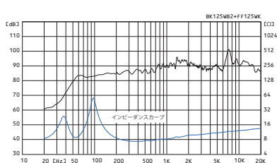
■周波数特性：BK125WB2+FF125WK
