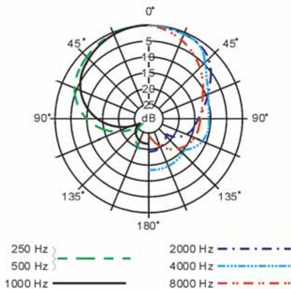
Polar Pattern
