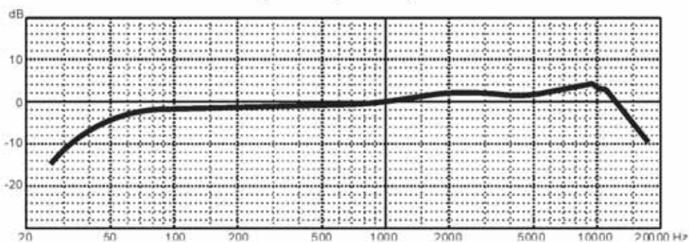
Frequency Response
